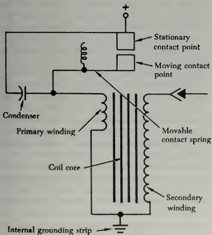
FIGURE 4-21. Booster coil schematic.
